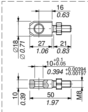
Spool end joint dimension
