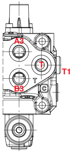
Centro chiuso Closed centre
